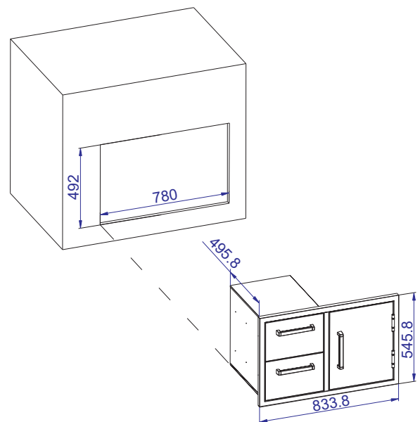
Cutout Size
