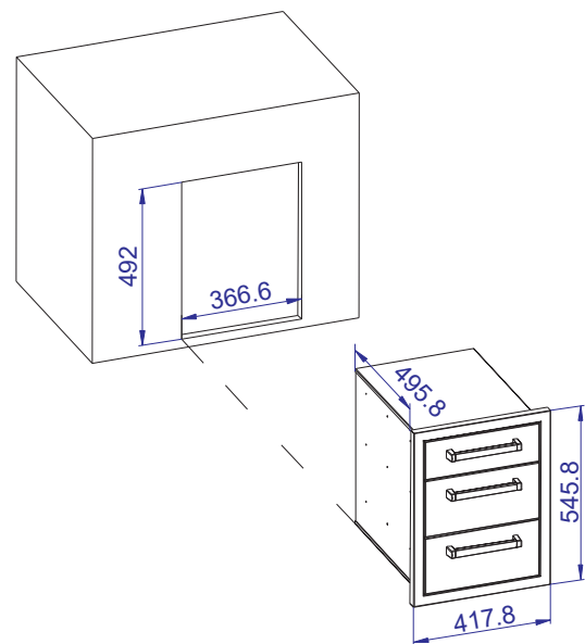
Cutout Size
