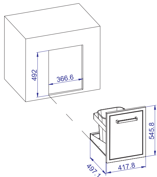
Cutout Size
