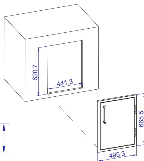
Cutout Size
